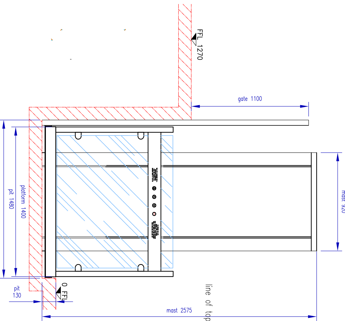
SECTION 'D'- 'D' LIFT AT LOWER LEVEL
